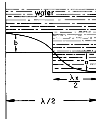
Fig. 5. Fluid configuration analyzed in Fermi's model.
