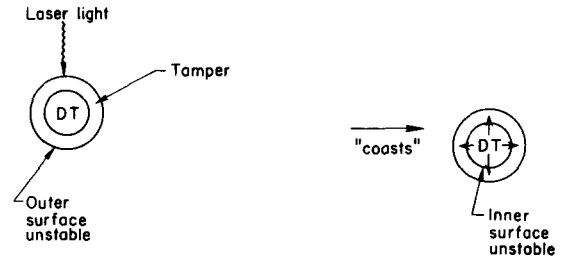
Fig. 2. Schematic diagram of the implosion of DT pellet.
